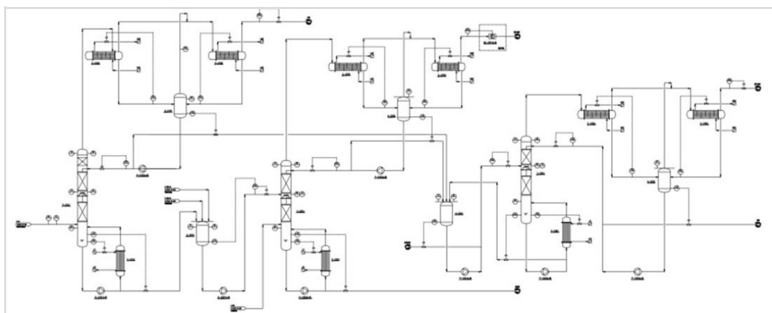
Solvent Recovery Three-Column Process
