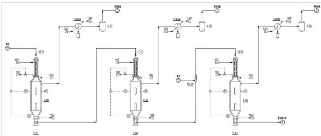
three-stage DSXL Devolatilization diagram
